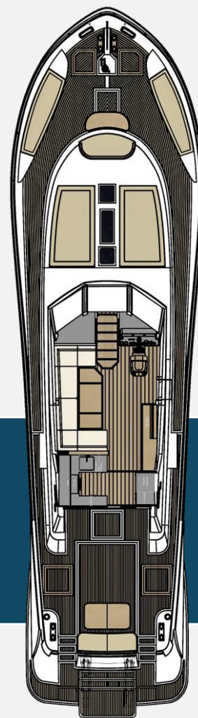
Main Deck
